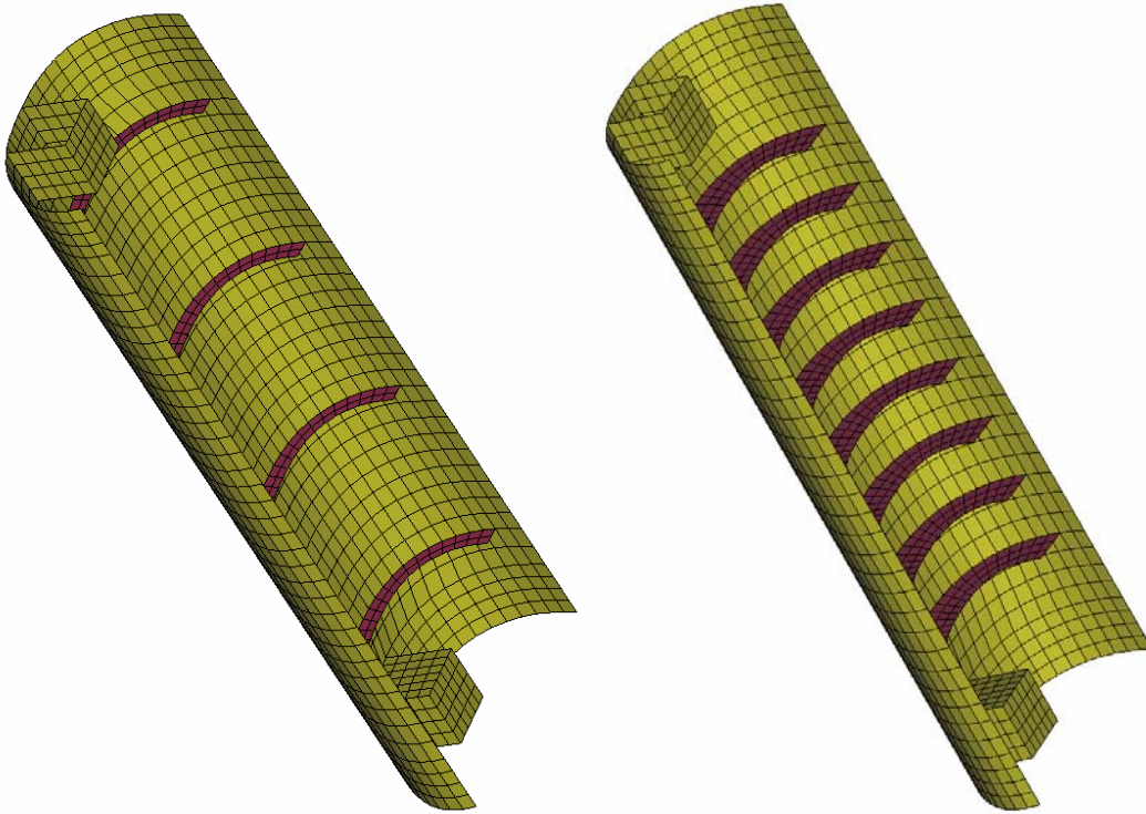
Figure 7: Baseline (left) and Optimal (right) designs
