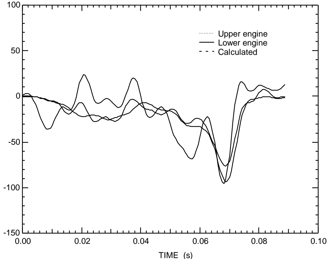
Figure 5. Measured and calculated engine accelerations in the frame impact test.
