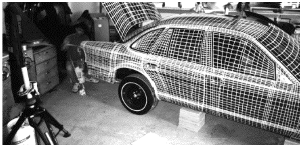
(b) Vehicle tear-down and digitization.
