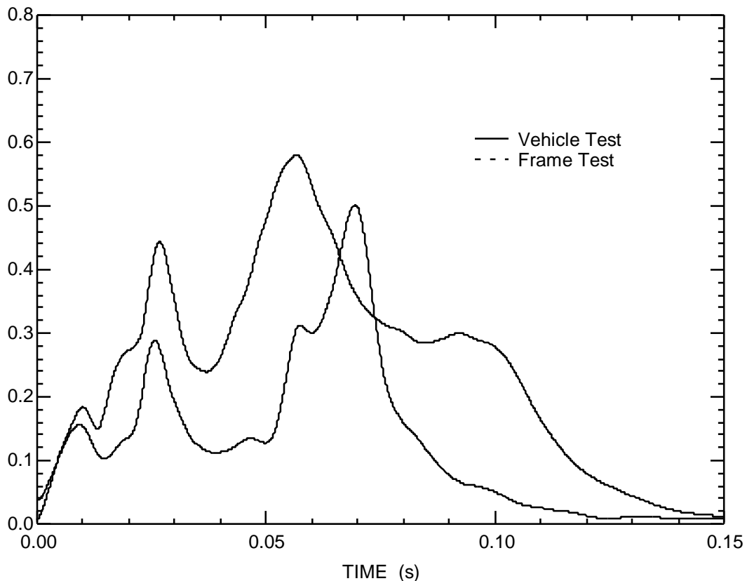
Figure 4. Comparison of the vehicle and frame frontal barrier impact tests.
