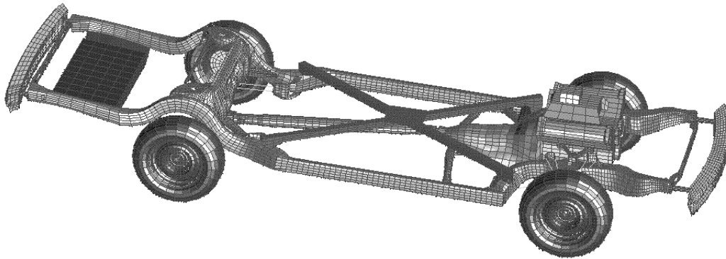
Figure 3. Model of the frame and drivetrain used in the 56 km/hr.
