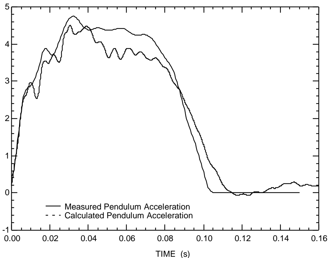
Figure 6. Measured and calculated pendulum accelerations in the bumper impact test.
