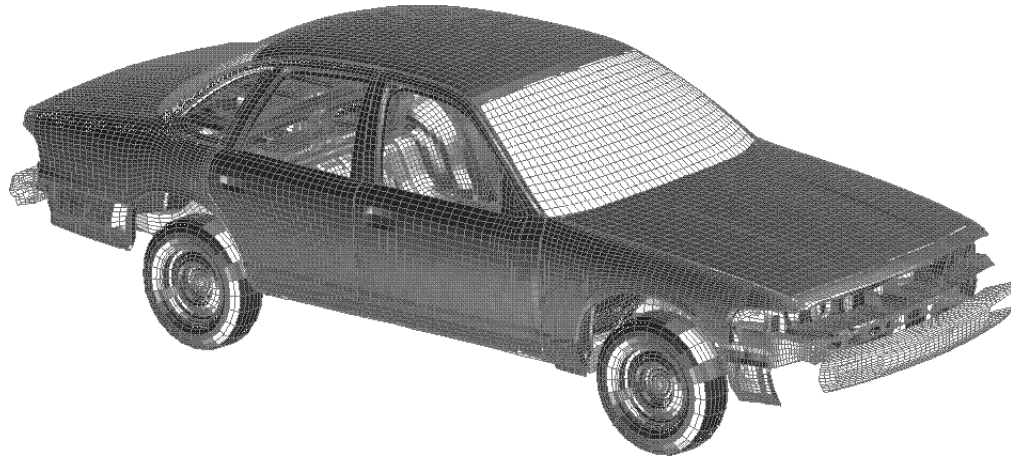
(a) Vehicle front view.
