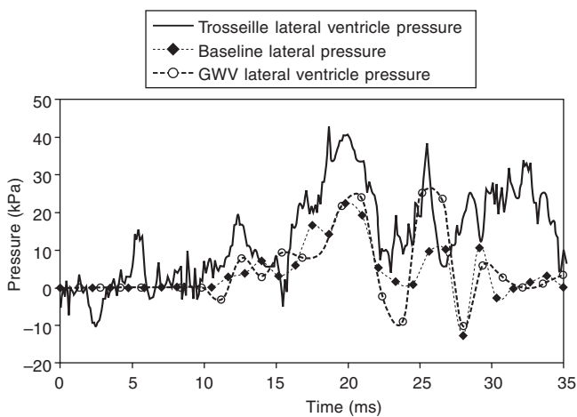
Figure 11 Comparison of experimental and simulated pressures at the lateral ventricle for the baseline and the GWV model. Pressure is measured at the same element for both models.
