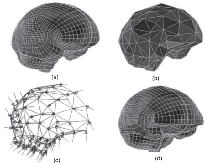
Figure 8 Steps used to make the morphed model. A coarse grid (b) was constructed on the original model (a). A discrete field of displacement vectors was then applied to every node of this coarse grid (half of which are visible in (c)), and this field was converted into a continuous field in order to create (d). The morphed model is of Van Lierde and Vander Sloten [42] while the original model is of the visible male [32].
